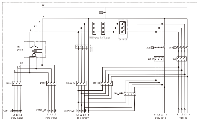
STS100D CABINET
